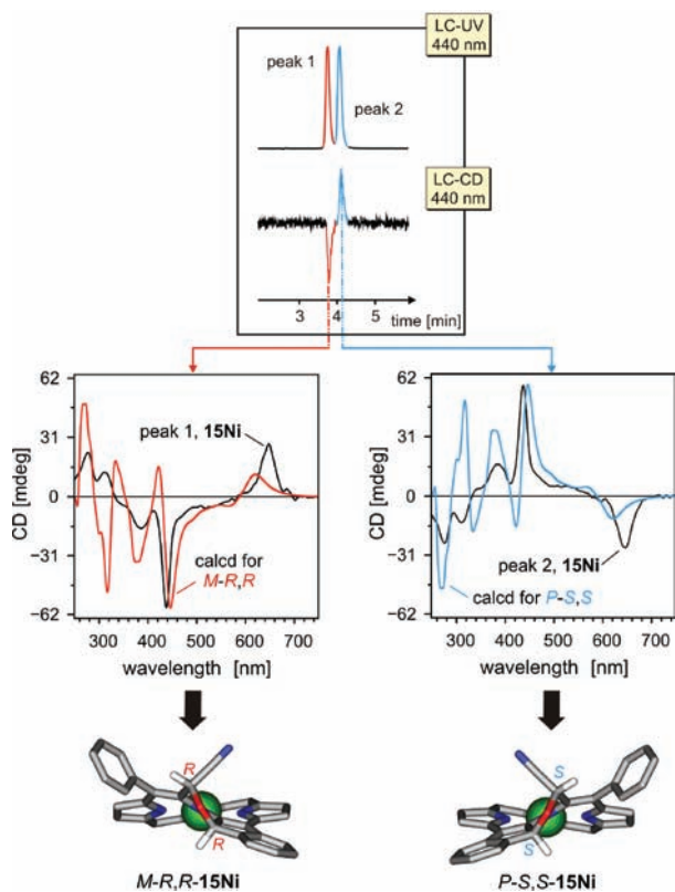
Figure 7. Results of the HPLC resolution of a racemic mixture of 15Ni (Chirex-3010 column, Phenomenex; ambient temperature; n -hexane- \text{CH}_2\text{Cl}_2 (v/v) 50:50, isocratic flow: 1.5 mL/min) and stereochemical assignment of the two enantiomers by comparison of the experimental CD spectra with the computed ones. 45 The rear phenyl substituents and all hydrogens located at \text{sp}^2 -carbon atoms were omitted for clarity.
